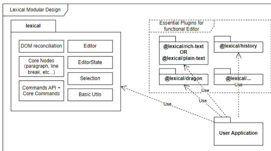
รูป 2.5 Lexical modular design
