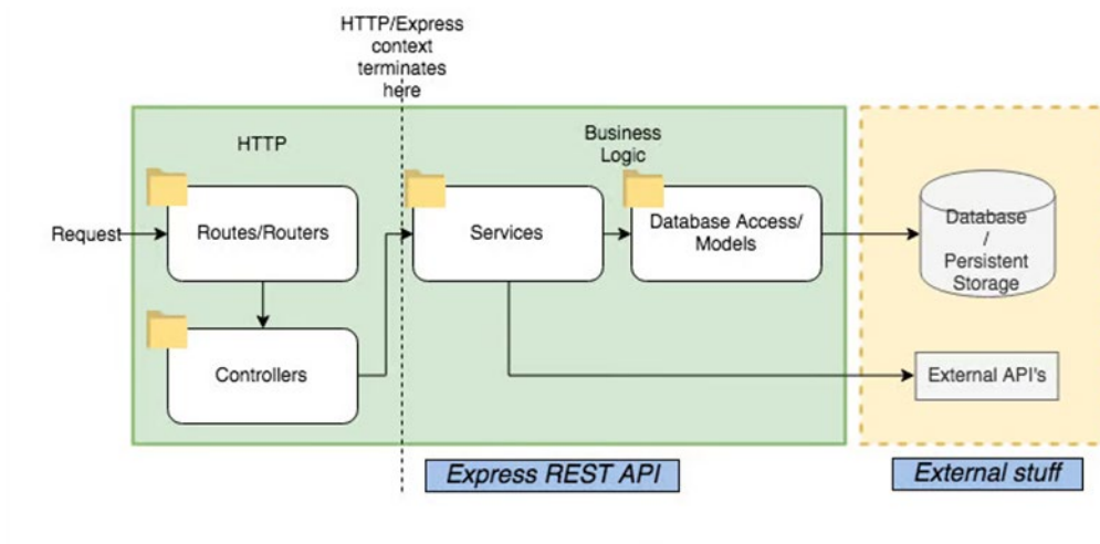
รูป 2.6 Express Architecture Diagram
