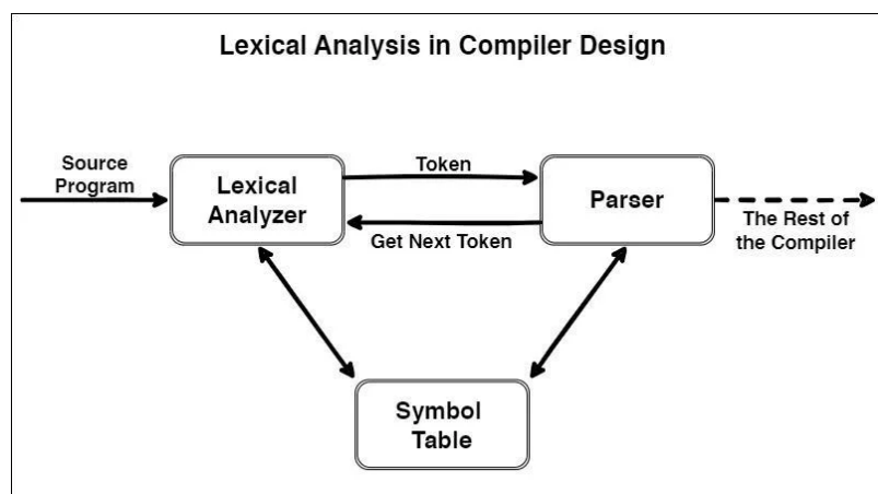
รูป 2.1 Lexical Analysis in Compiler Design
